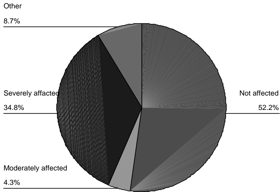
Figure 8. Percentage of authors giving each category of response to whether recoding country of birth from 42 categories to two would affect their analyses
